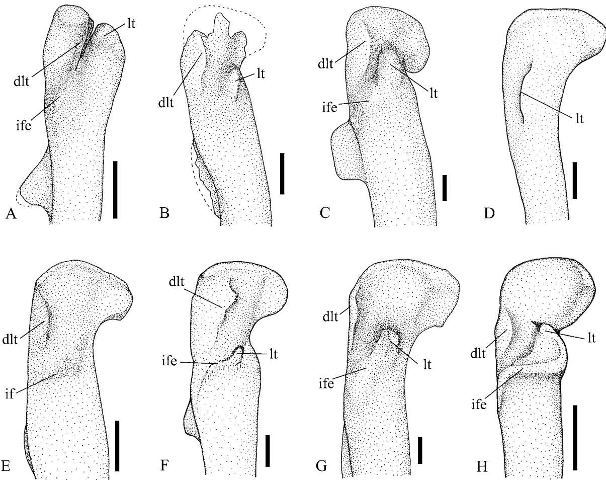
Figure 12 Lateral aspect of proximal femur of A , Lesothosaurus diagnosticus , right femur based on BMNH RUB17; B , Guaibasaurus candelariensis , right femur based on MCN-PV 2355; C , Efraasia diagnostica , right femur based on SMNS 12684; D , cf. Massospondylus carinatus , left (reversed) femur based on BPI 5006; E , Staurikosaurus pricei , left (reversed) femur based on MCZ 1669; F , Herrerasaurus ischigualastensis , right femur based on PVSJ 373; G , Liliiensternus liliiensterni , left (reversed) femur based on MB R.1275; H , Syntarsus rhodesiensis , left (reversed) femur based on QVM QG 174; Abbreviations: dlt , 'dorsolateral trochanter'; ife , insertion of M. iliofemorale ; ife , insertion of M. iliofemoralis externus ; lt , 'lesser trochanter'. Scale bars: A = 10 mm, B–H = 20 mm.
