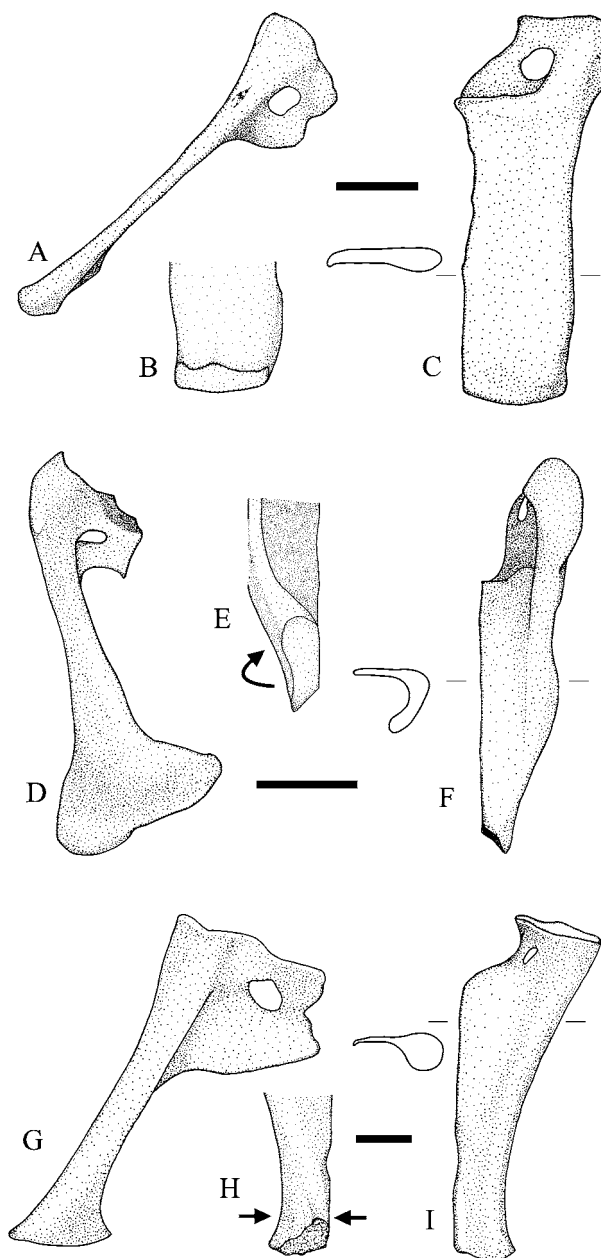
Figure 10 Pubis of A–C , Plateosaurus engelhardti , left pubis based on GPIT 'skelett 2' and Yates (2003b); D–F , Herrerasaurus ischigualastensis , right (reversed) pubis, based on PVL 2566 and Novas (1993); G–I , Torvosaurus tanneri , right (reversed) pubis, based on Galton & Jensen (1979). Lateral ( A , D , G ) and cranial, with outline of transverse section ( C , F , I ), aspects of the pubis and distal pubis in caudal aspect ( B , E , H ). Arrows approximately indicate the change required for the distal pubis of Plateosaurus to acquire a shape like that of Herrerasaurus and Torvosaurus . Scale bars = 100 mm.
