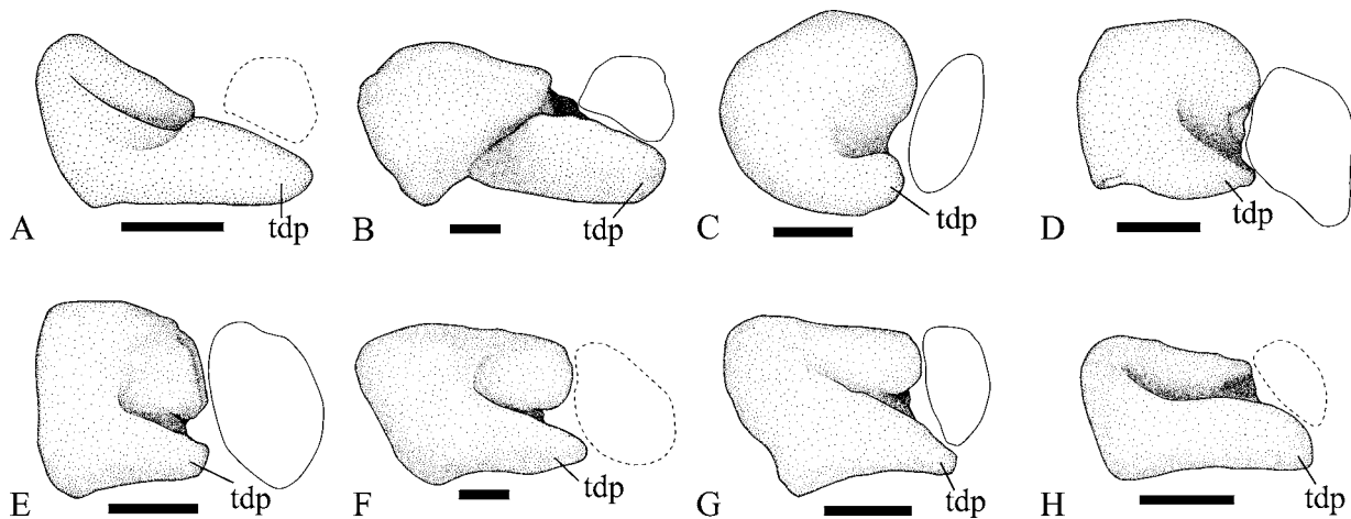
Figure 13 Distal tibia and outline of distal fibula of A , cf. Lesothosaurus diagnosticus , right tibia (reversed) based on BMNH R11001; B , Scelidosaurus harrisonii , right (reversed) tibia and fibula based on BMNH 1111; C , Staurikosaurus pricei , left tibia and fibula based on MCZ 1669; D , Herrerasaurus ischigualastensis , left tibia and fibula based on PVSJ 373; E , Saturnalia tupiniquim , right (reversed) tibia and fibula based on MCT 3944PV; F , cf. Riojasaurus incertus , right (reversed) tibia based on PVL 3525; G , Liliensternus liliensterni , left tibia and fibula based on MB R.1275; H , Syntarsus rhodesiensis , left tibia based on QVM QG 792. Abbreviations: tdp , descending process of tibia. Scale bars: A, C, E, H = 10 mm; B, D, F, G = 20 mm.
