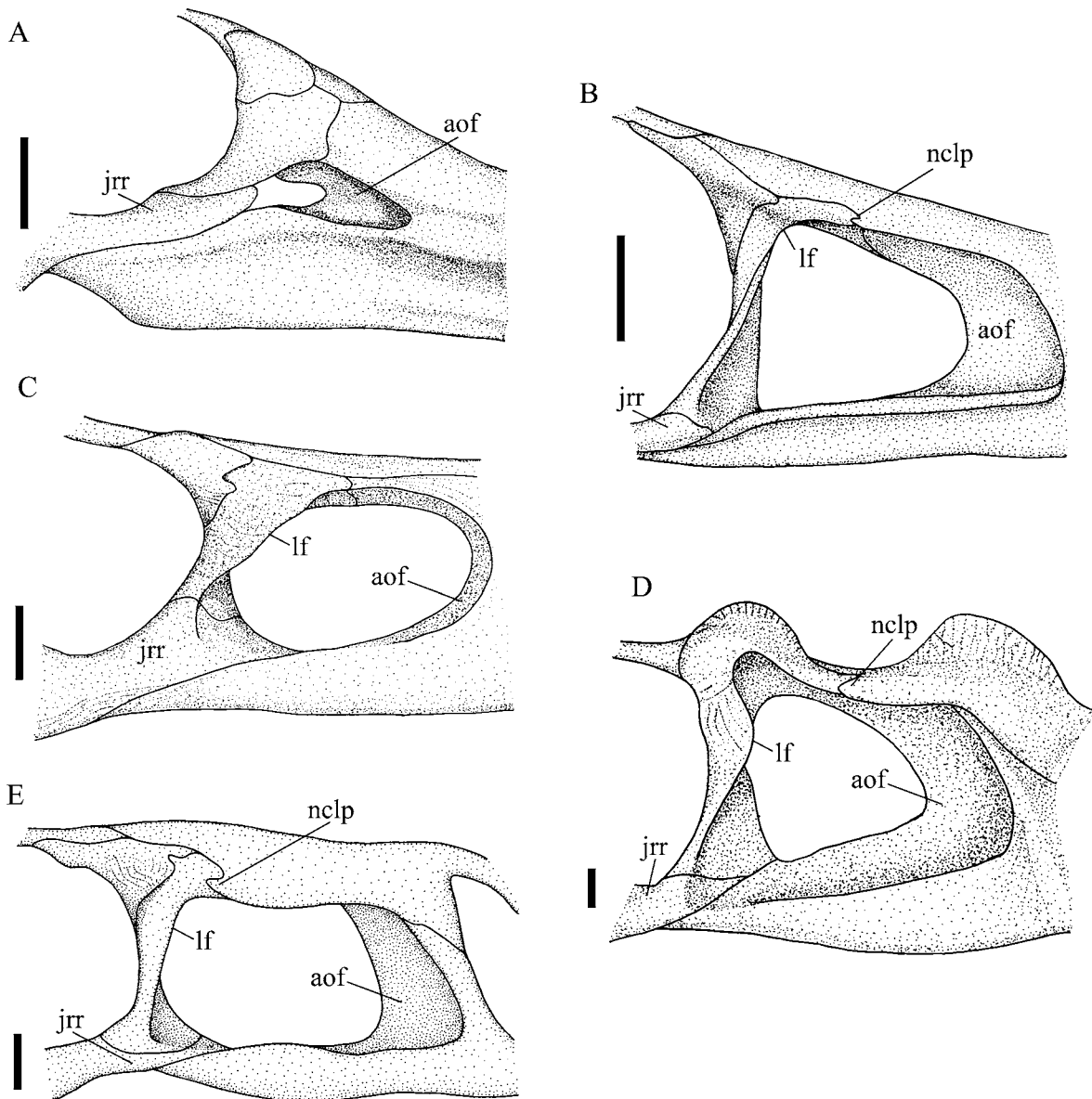
Figure 5 Lateral aspect of the orbital portion of the skull of A , Scelidosaurus harrisonii , based on BMNH 1111; B , Eoraptor lunensis , based on PVSJ 512 and Sereno et al. (1993); C , Herrerasaurus ischigualastensis , based on PVSJ 407 and Sereno & Novas (1994); D , Ceratosaurus magnicornis , based on Madsen & Welles (2000); E , Plateosaurus engelhardti , based on Galton (1984a). Abbreviations: aof , antorbital fossa; jrr , jugal rostral ramus; lf , lacrimal flange; nclp , nasal caudolateral process. Scale bars: A, C–E = 20 mm; B = 10 mm.
