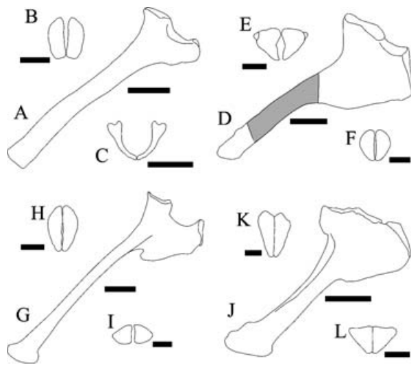
Figure 11 Ischium of A , Scelidosaurus harrisonii , based on BMNH 6704; B , cf. Lesothosaurus diagnosticus , based on BNHM R 11001; C , Lesothosaurus diagnosticus , based on Thulborn (1972); D , E , Herrerasaurus ischigualastensis , based on Novas (1993; shading represents unpreserved portion); F , Staurikosaurus pricei , based on MCZ 1669; G – I , Syntarsus rhodesiensis , based on Raath (1969, 1990); H , Coelophysis sp., based on Padian (1986); J – K , Plateosaurus engelhardti , based on Huene (1926) and Yates (2003b); L , Massospondylus carinatus , based on Cooper (1981). Lateral ( A , D , G , J ) and distal ( B , E , H , K ) aspects, with outlines of mid-shaft cross-section ( C , F , I , L ). Scale bars: A , E , G , H , L = 20 mm; B , C , F , I = 10 mm; D , K = 50 mm; J = 100 mm.
