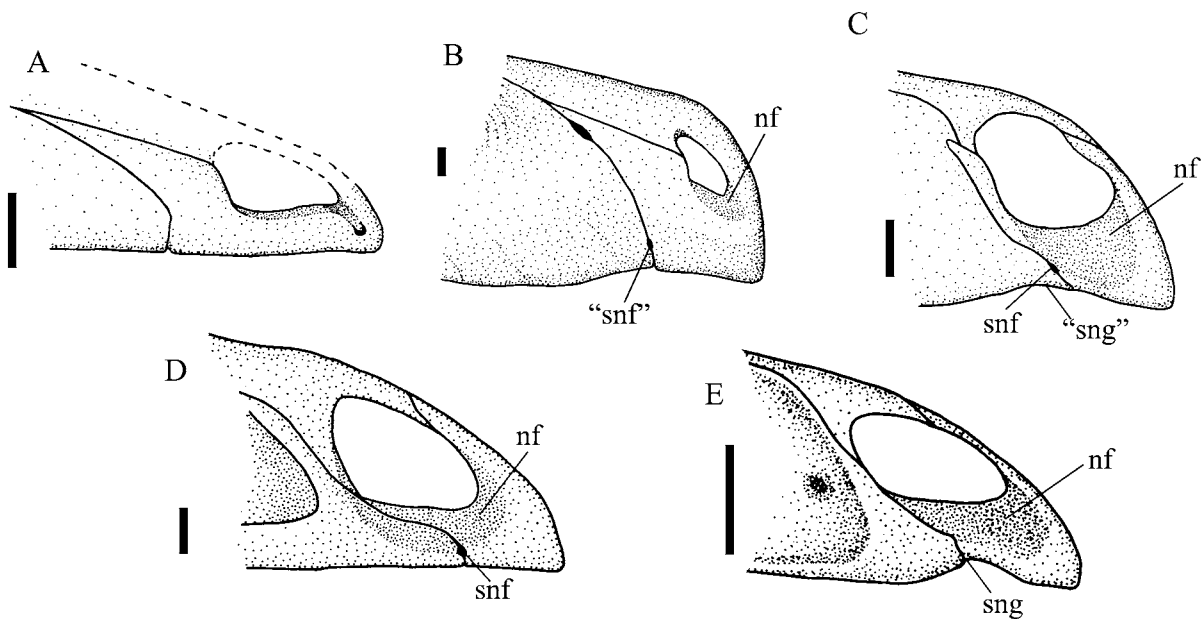
Figure 4 Lateral aspect of the rostral part of the skull of A , Lesothosaurus diagnosticus , based on BMNH R8501 and Sereno (1991b); B , Herrerasaurus ischigualastensis , based on PVSJ 407 and Sereno & Novas (1994); C , Eoraptor lunensis , based on PVSJ 512 and Sereno et al. (1993); D , Efraasia diagnostica , based on Yates (2003b); E , cf. Syntarsus rhodesiensis , based on BP/1/5278 and Munyikwa & Raath (1999). Abbreviations: nf , narial fossa; snf , subnarial foramen; sng , subnarial gap. Scale bars: A , C = 5 mm; B , D , E = 10 mm.
