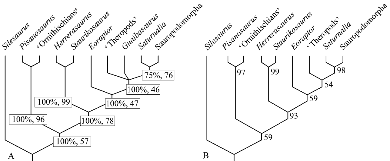
Figure 16 A , 'Majority rule' consensus of four most parsimonious trees (MPTs) found in the analysis of the data-matrix given in the Appendix applying the 'Emulate PeeWee' command of PAUP. B , Single MPT found in analyses of the data-matrix given in the Appendix, with the exclusion of Guaibasaurus . Clade statistics: percentage of MPTs in which the clade occurs (only in A ) and bootstrap values.
