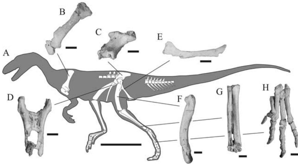
Figure 2 Skeletal reconstruction of Guaibasaurus candelariensis . A , preserved bones on shaded outline; B , left scapulocoracoid in lateral aspect; C , right ilium (reversed) in lateral aspect; D , pubic pair in cranial aspect; E , left ischium in lateral aspect; F , right femur (reversed) in lateral aspect; G , right tibia and fibula in cranial aspect; H , left pes in cranial aspect. B–G based on MCN-PV 2355 and H based on MCN-PV 2356. Scale bars: A = 250 mm; B–H = 25 mm.
