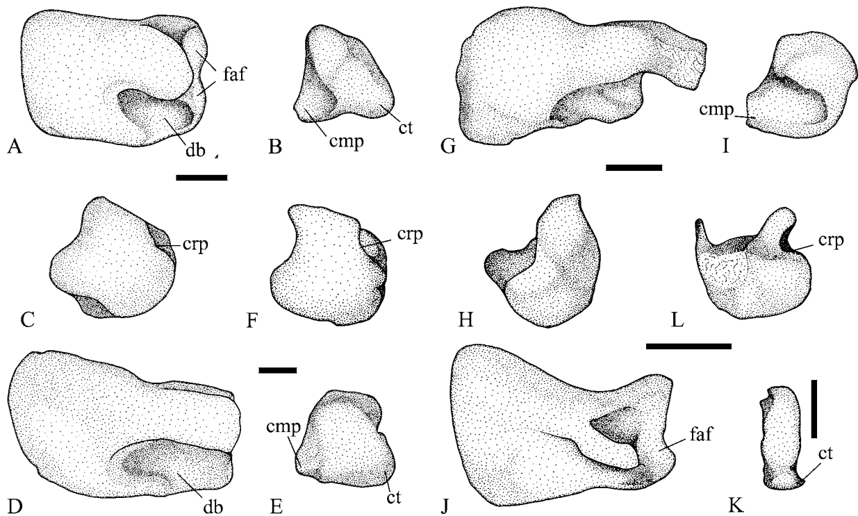
Figure 14 Tarsal bones of A–C , Herrerasaurus ischigualastensis , left astragalus (reversed) and right calcaneum based on PVL 2566; D–F , Plateosaurus engelhardti , left (reversed) tarsus based on GPIT ‘skelett 2’; G–I , Scelidosaurus harrisonii , right tarsus based on BMNH 1111; J–L , Syntarsus rhodesiensis , right astragalus based on QVM QG-CT-6 and left calcaneum (reversed) based on QVM unnumbered. Proximal ( A, B, D, E, G, I, J, K ) and lateral ( C, F, H, L ) aspects. Abbreviations: cmp , calcaneal medial process; crp , astragalus cranial platform; ct , calcaneal tuber; db , astragalus dorsal basin; faf , fibular articulation facet on astragalus. Scale bars: A–I = 20 mm; J–L = 10 mm.
