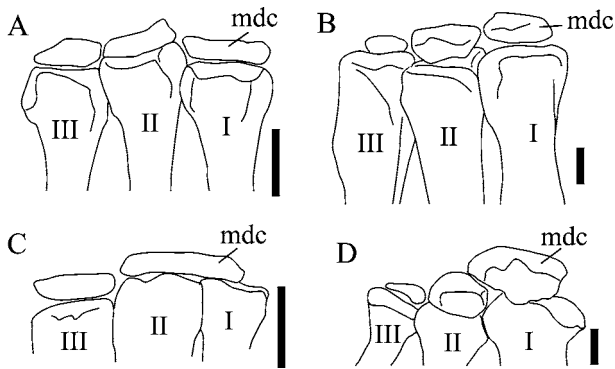
Figure 8 Extensor aspect of the proximal portion of metacarpals I–III and ‘correspondent’ distal carpals of A , Heterodontosaurus tucki , right manus based on Santa Luca (1980); B , Herrerasaurus ischigualstensis , left (reversed) manus based on Sereno (1994); C , Coelophysis bauri , left (reversed) manus based on Colbert (1989); D , Plateosaurus engelhardti , right manus based on SMNS ‘ Pachysaurus ajax ’. Abbreviations: I–III , Metacarpals I–III; mdc , medial-most distal carpal. Scale bars = 5 mm.
