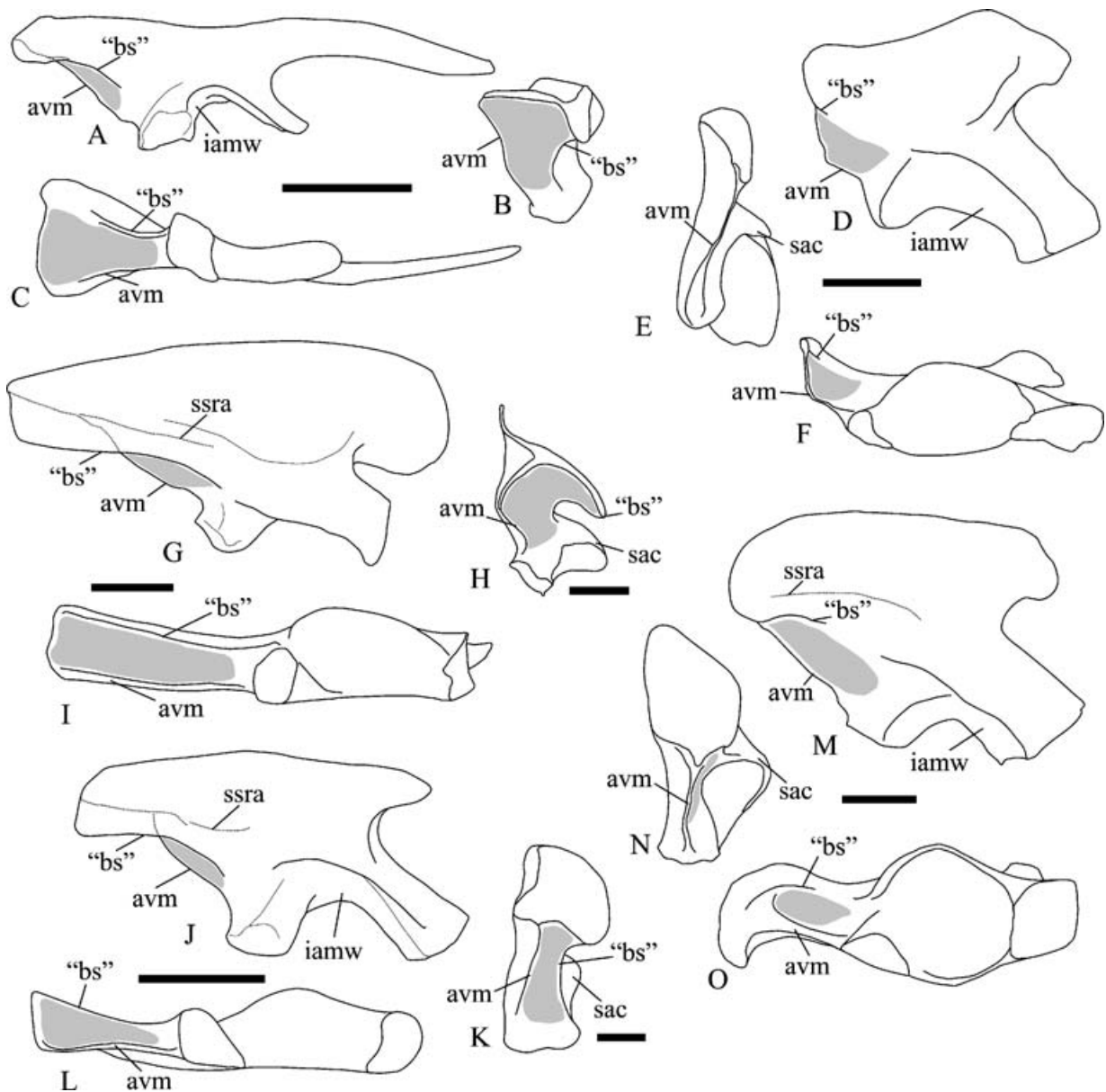
Figure 9 Ilium of A–C , Dryosaurus lettowvorbecki , based on MB dy II and III and Galton (1981); D–F , Staurikosaurus pricei , based on MCZ 1669; G–I , theropods, based on Liliensternus liliensterni (MB R.1275) ( G and I ) and Elaphrosaurus bambergi (MB ‘mounted skeleton’ and Janensch, 1925) ( H ); J–L , ‘Prosauropods’, based on Efraasia diagnostica (SMNS 12684, 12667, and Galton 1973) ( J and L ), and Plateosaurus engelhardti (SMNS 13200) ( K ); M–O Herrerasaurus ischigualastensis , based on PVL 2566 and Novas (1993). Lateral ( A , D , G , J , M ), caudal ( B , E , H , K , N ) and ventral ( C , F , I , L , O ) aspects. Abbreviations: avm , ventral margin of caudal ala; ‘bs’ ‘brevis shelf’; iamw , medial wall of iliac acetabulum; sac , supraacetabular crest; ssra , dorsal margin of second sacral rib articulation; ‘shading’ , hypothesised origin area of M. caudofemoralis brevis . Scale bars = 50 mm.
