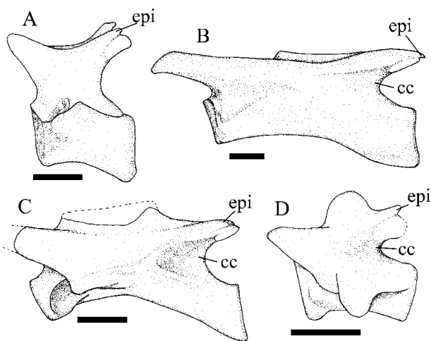
Figure 6 Lateral aspect of post-axial cranial cervical vertebrae of A , Lesothosaurus diagnosticus , third cervical vertebra based on BMNH R11004; B , Plateosaurus engelhardti , third cervical vertebra based on SMNS F65; C , Liliiensternus liliiensterni , third? cervical vertebra based on MB R.1275; D , Staurikosaurus pricei , fourth? cervical vertebra based on MCZ 1669. Abbreviations: cc , caudal chonos; epi , epiphysis. Scale bars: A = 5 mm; B–D = 20 mm.
