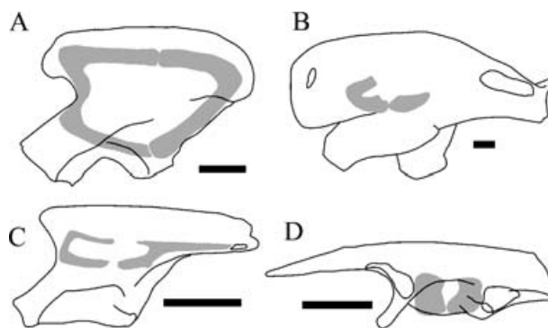
Figure 7 Lateral outlines of ilium and sacral vertebrae articulations of A , Herrerasaurus ischigualastensis , based on PVL 2566 and Novas (1993); B , Dilophosaurus wetherilli , based on Welles (1984); C , Saturnalia tupiniquim , based on MCT 3944PV; D , Scelidosaurus harrisonii , based on BMNH 6704. Primordial sacral vertebrae articulations in grey. Scale bars: A = 50 mm, B–D = 30 mm.
