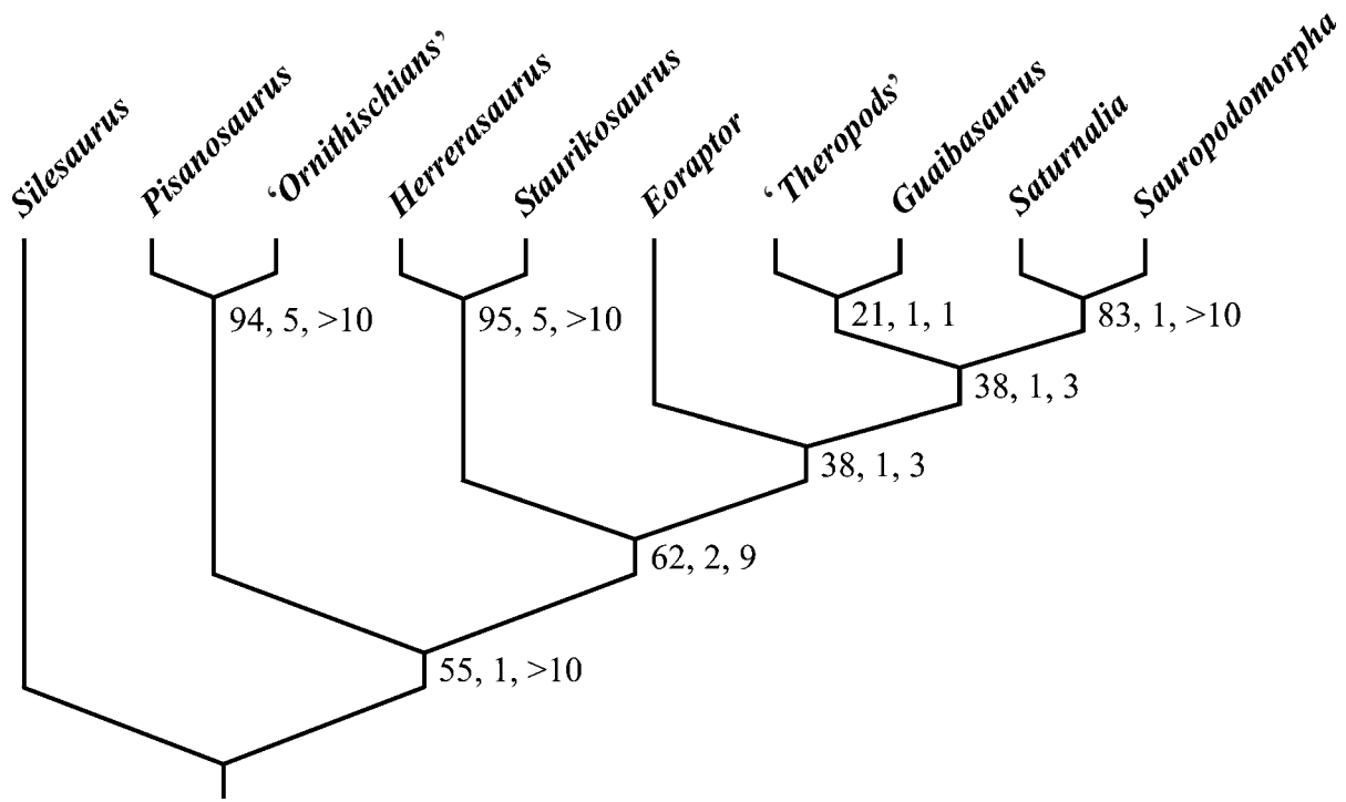
Figure 15 Single 'most parsimonious tree' (MPT) of 203 steps found in the analysis of the data-matrix given in the Appendix. Clade statistics are, respectively, bootstrap value, 'strict' and 'majority rule' values of Bremer support.
