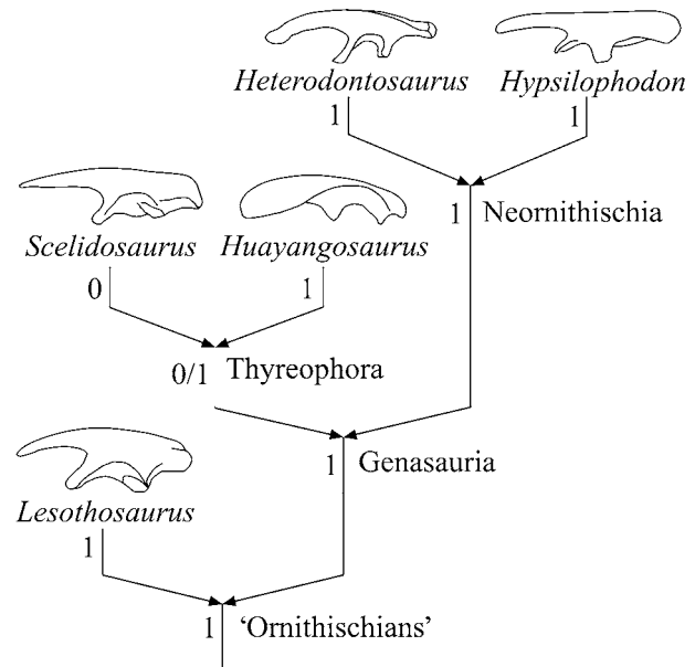
Figure 1 The ‘outgroup algorithm’ used to trace morphological changes and infer character states of composite ingroup operational taxonomic units (OTUs). In this case, exemplified by the acetabular aperture of ornithischians, it is based on the phylogeny of Sereno (1999). Abbreviations (character states): 0, closed acetabulum; 1, semi-perforated acetabulum.
