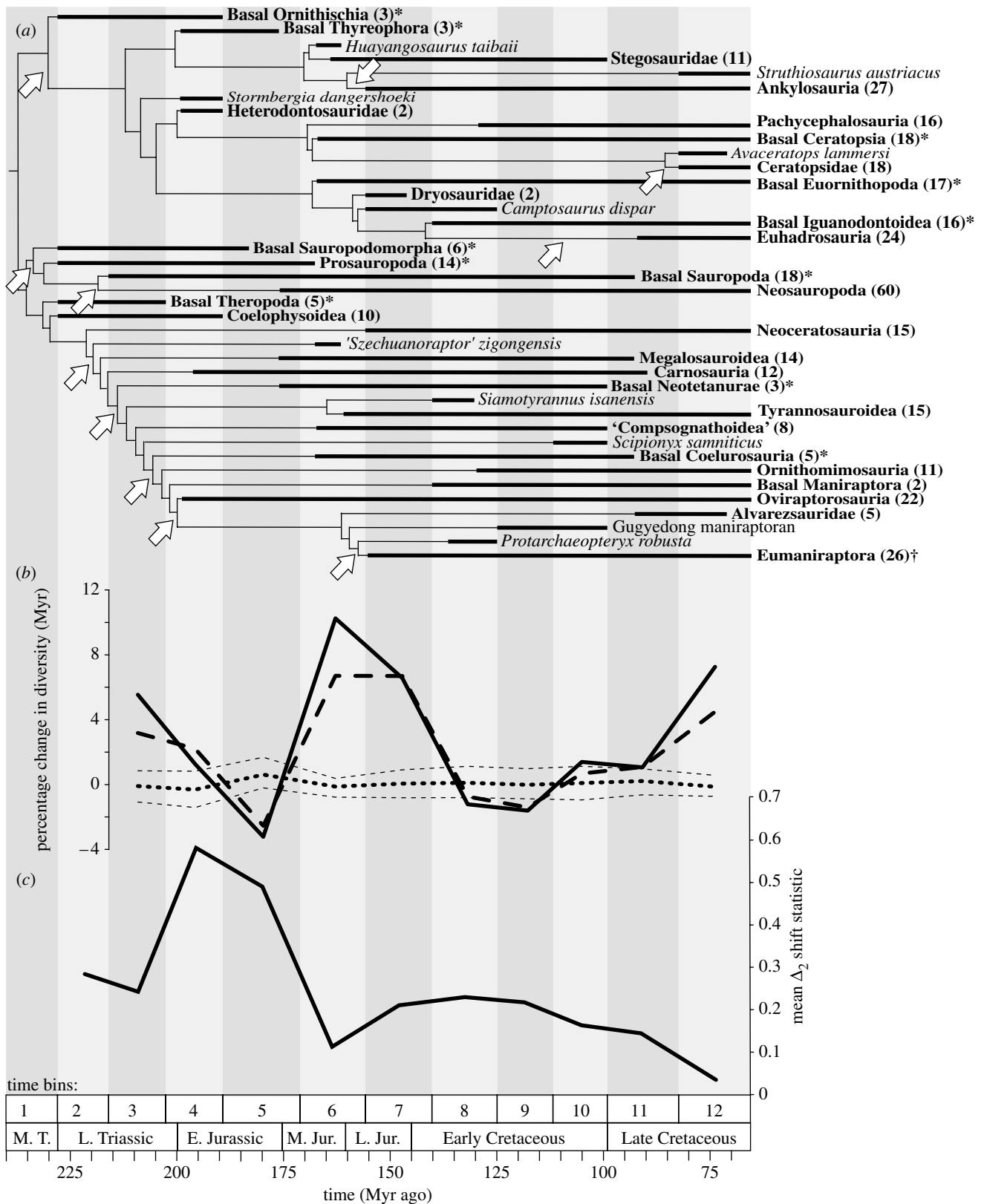
Figure 2. Results of different analyses of dinosaur diversification. (a) A summary version of the supertree used here; the 11 statistically significant diversification shifts present in both the entire tree and at least one time slice are marked with white arrows denoting the branch leading to the more speciose clade. Taxa in bold represent the collapsing of a larger clade, the size of which is indicated in parentheses. An ‘*’ indicates the collapsing of a paraphyletic group and a ‘†’ that of an extant clade (i.e. birds). (b) Diversification rates based on the raw record (solid line), the raw record plus additional ghost ranges (dashed line) and subsampled data (dotted lines; see text). (c) Mean values of \Delta_2 shift statistic through time (see text).
