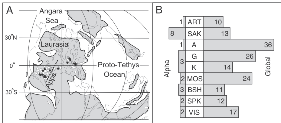
Figure 1. Data distribution. A: By paleogeography (300 Ma; after Scotese and McKerrrow, 1990). B: By stratigraphy. Open circles are global data and closed circles are alpha data. VIS—Viséan; SPK—Serpukhovian, BSH—Bashkirian, MOS—Moscovian, K—Kasimovian, G—Gzhelian, A—Asselian, SAK—Sakmarian, ART—Artinskian, Apps—Appalachians.
