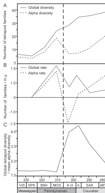
Figure 2. Tetrapod diversification patterns from Viséan (346 Ma) to Artinskian (270 Ma). A: Global diversity of tetrapods and alpha diversity. B: Alpha and global diversification rates measured as first derivative of values in A. C: Endemism measured as global diversity ( T_1 ) divided by mean alpha diversity ( \bar{T} ) (Sepkoski, 1988). Vertical dotted line highlights Moscovian-Kasimovian boundary. Time scale after Davydov et al. (2010). Abbreviations as in Figure 1.
