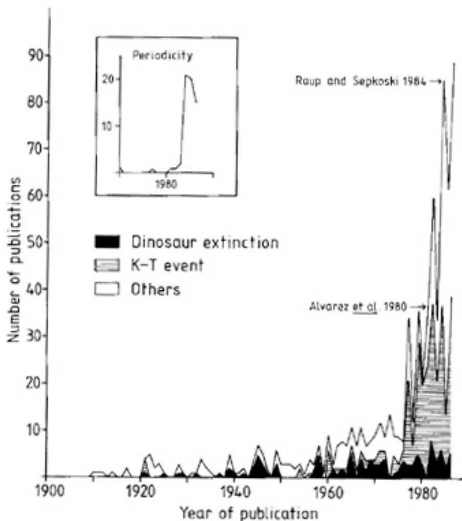
FIG. 1. The increasing rate of publication on dinosaur extinction, and the K-T event, from 1900 to 1986. Figures are plotted Year by year, based on a compilation of publications that are concerned solely or mainly with dinosaur extinction, with the K-T event (including stratigraphic accounts), and with broad questions of extinction that relate to the K-T event (shown as "others"). Since 1980, most of the publications that fall in the last category concern the periodicity debate, and these are also plotted separately in the inset. Two seminal papers, in 1980 and 1984, are noted in the diagram.
